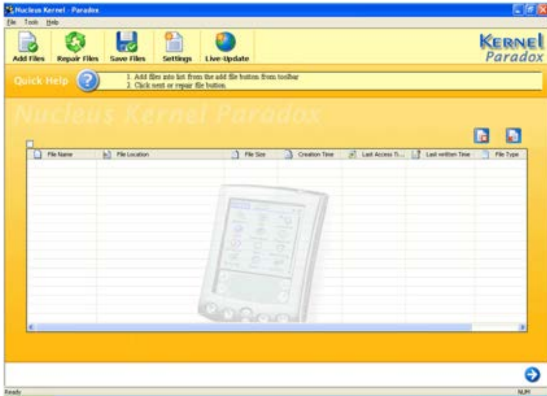
Figure 4.1: Main Window
